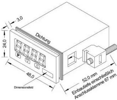
Dimensional drawing 1
