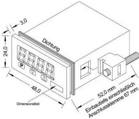
Dimensional drawing 1
