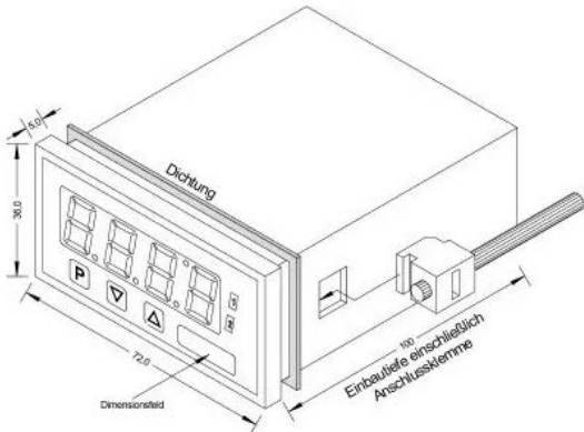
Dimensional drawing 1
